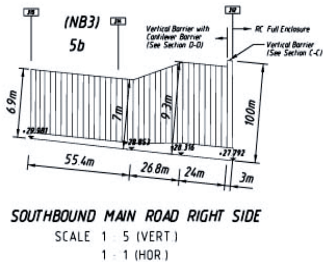
Route 8 - West Kowloon to Shatin - Entrusted Portion Figure 2.3 – R.C. Full Enclosure Entrance (Extracted from the Application VEP-249/2008)
